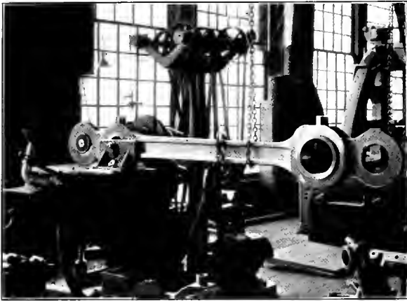
Fig. 5—Grinding Knuckle Pin Bushings in Side Rods
